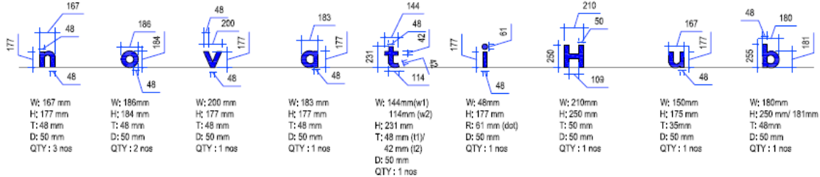
SIGNAGE ELEVATION DETAIL
